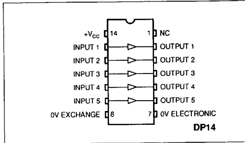
Figure 1: Pin connections (viewed from underside)
