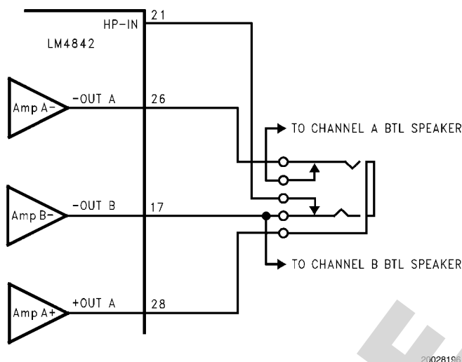
FIGURE 5. Headphone Sensing Circuit
