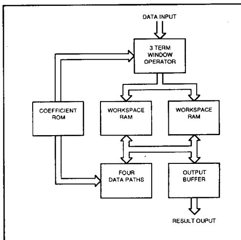
Fig. 1. Block Diagram
