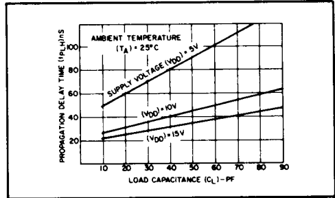
Typical propagation delay time vs. C_L -complement output.
