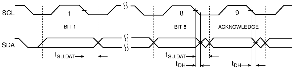
Figure 4. Serial Bus Timing
