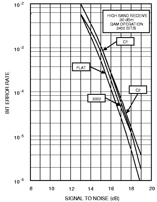
73K324BL BER VS S/N-QAM-HIGH BAND
