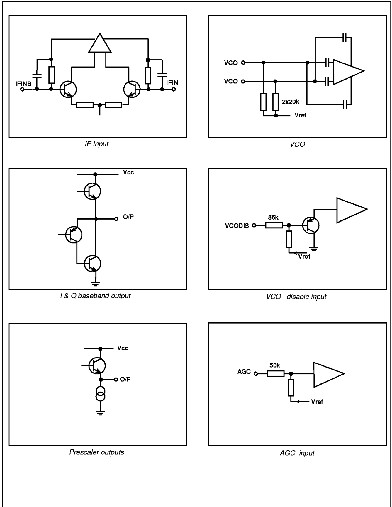
Fig. 6 I/O port peripheral circuitry
