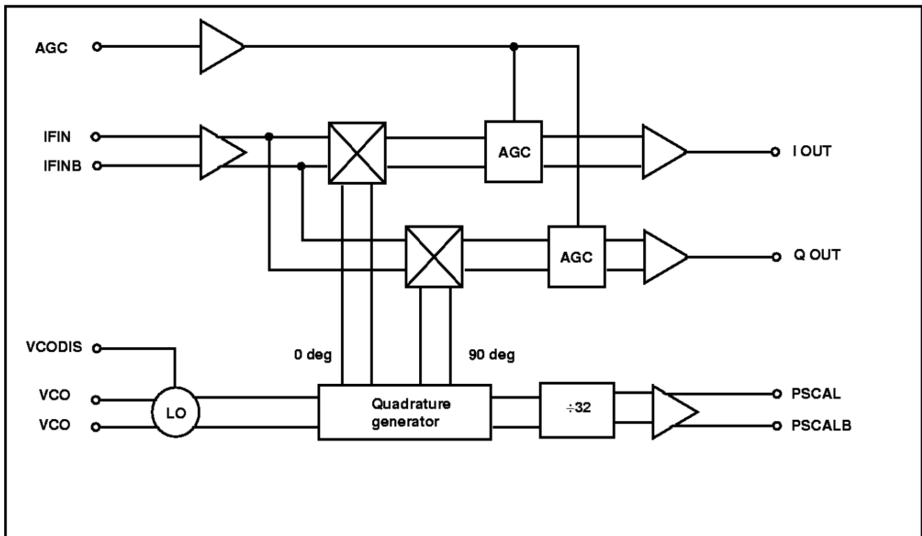
Fig. 2 SL1714 block diagram
