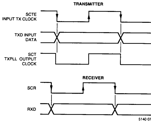
Figure 6. SC11045/SC11055 Synchronous Mode Timing Diagrams
