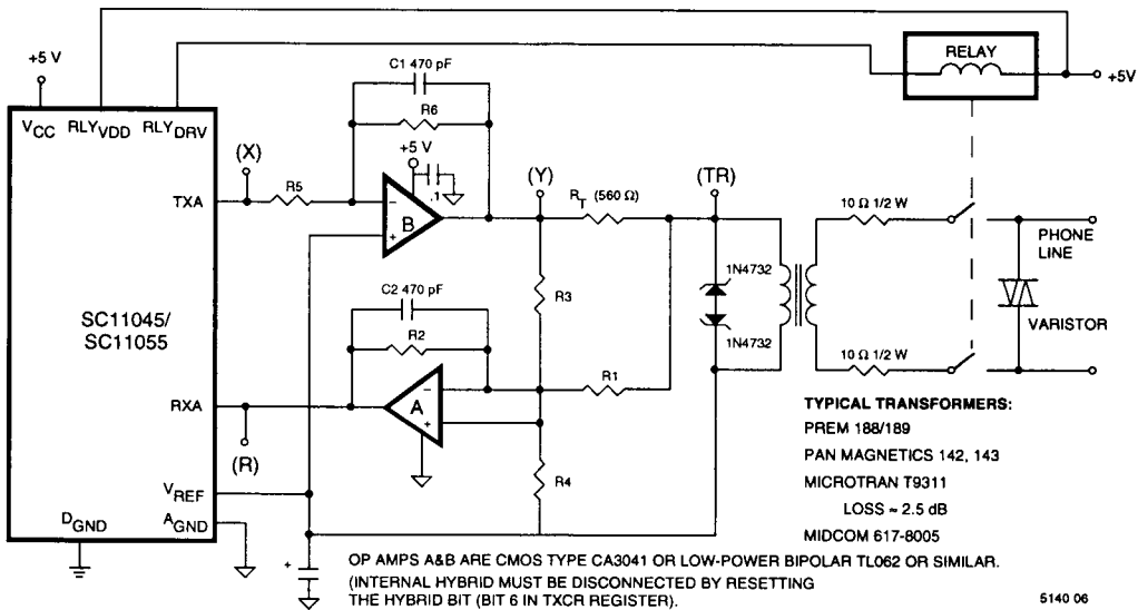
Figure 4. Using an External Hybrid with the SC11045/SC11055
