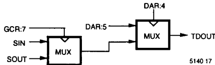
Figure 5e. TDOUT Function
