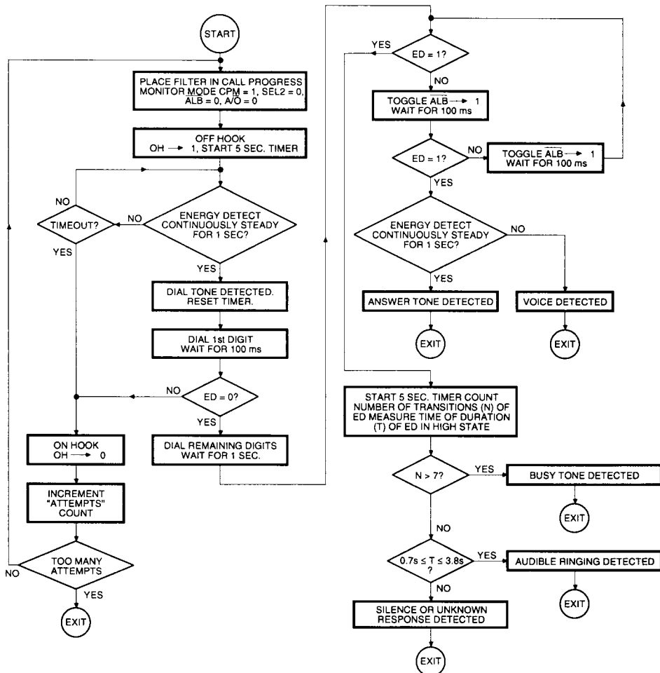
Figure 17. Call Progress Monitoring Algorithm
