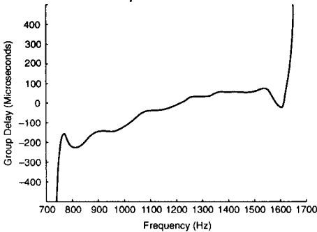
Figure 4. Low-Band Group Delay
