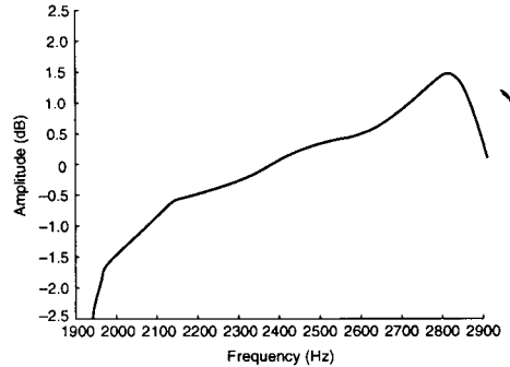
Figure 5. High-Band Response—Normalized
