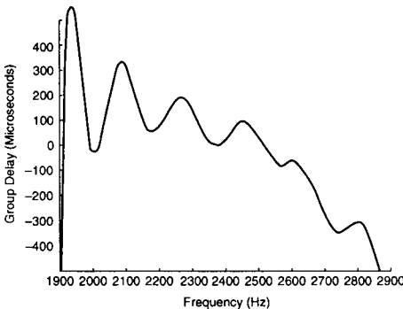
Figure 6. High-Band Group Delay (Hz)
