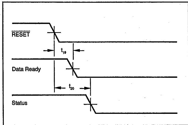
ADC700 Reset Function Timing Diagram.
