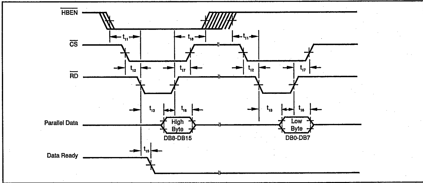
ADC700 Parallel Output Timing.
