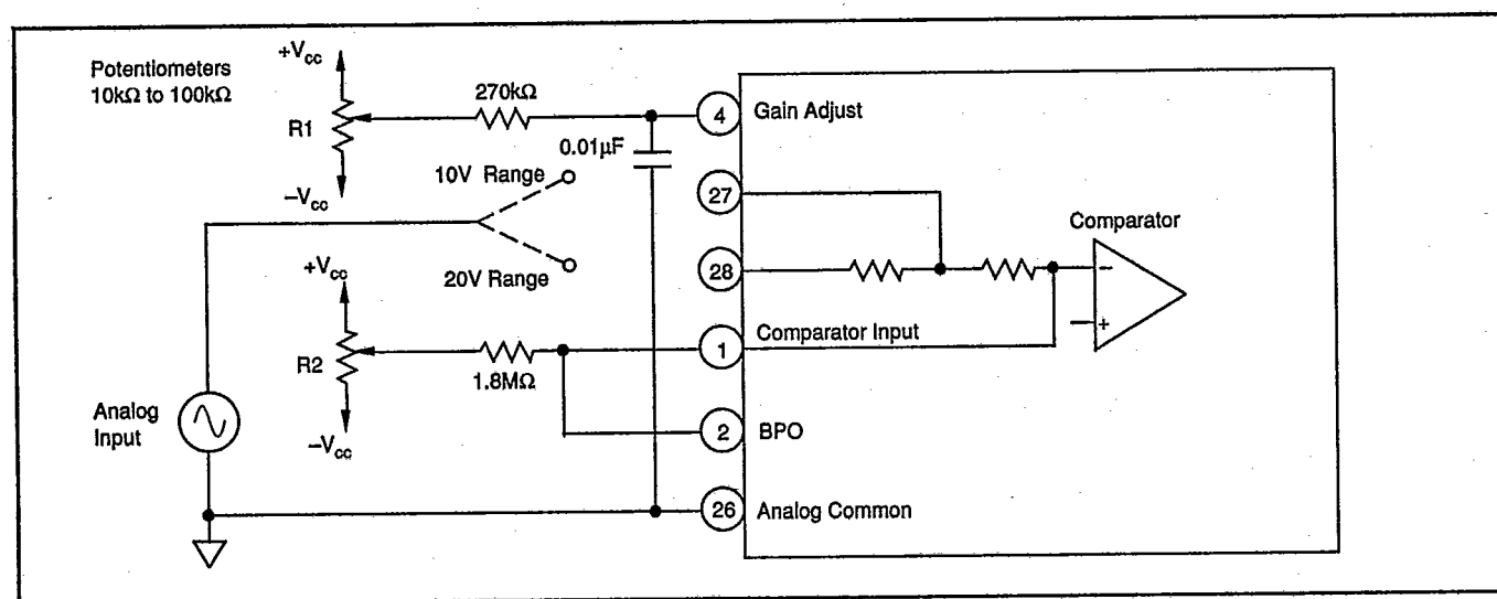
FIGURE 7. Bipolar Input Configuration with Gain and Offset Adjust Connections.
