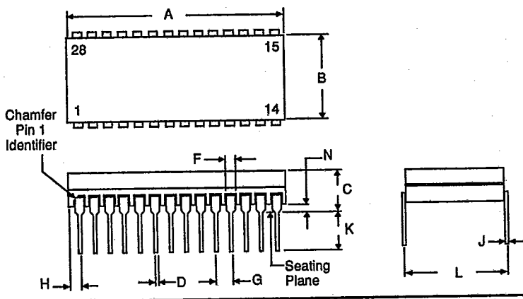
H Package — 28-Pin Ceramic DIP
