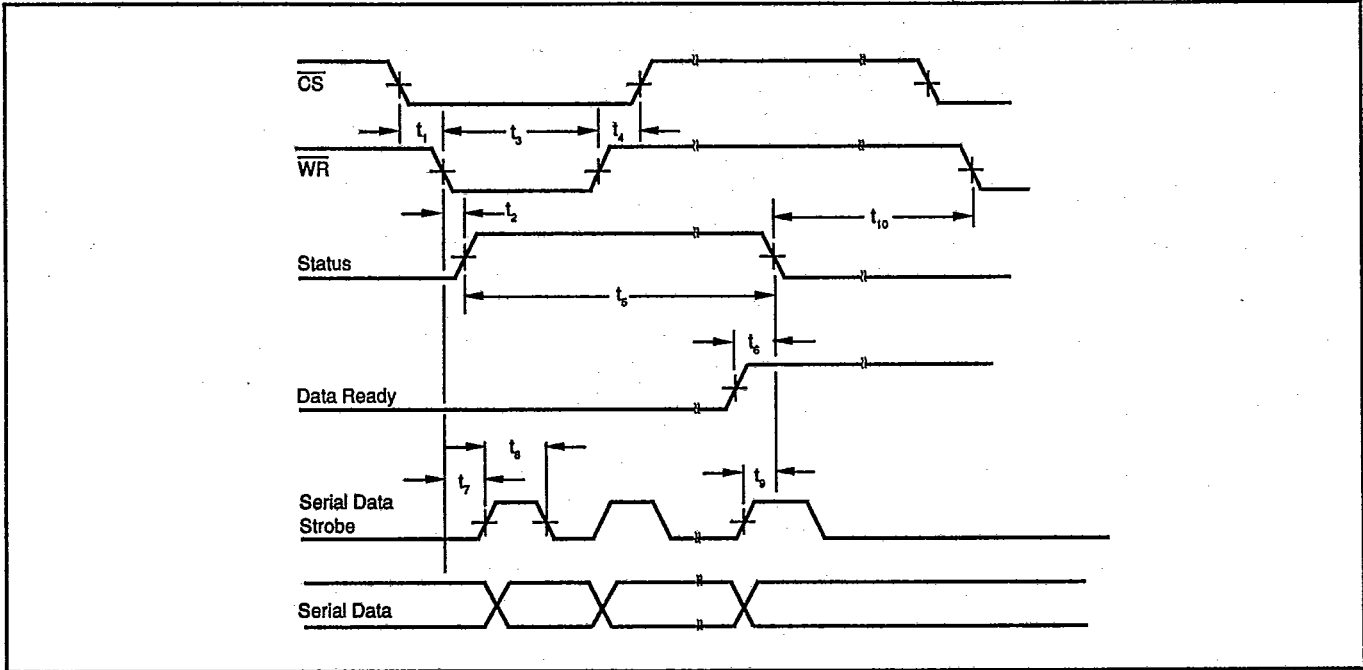
Start of Conversion and Serial Data Output Timing.
