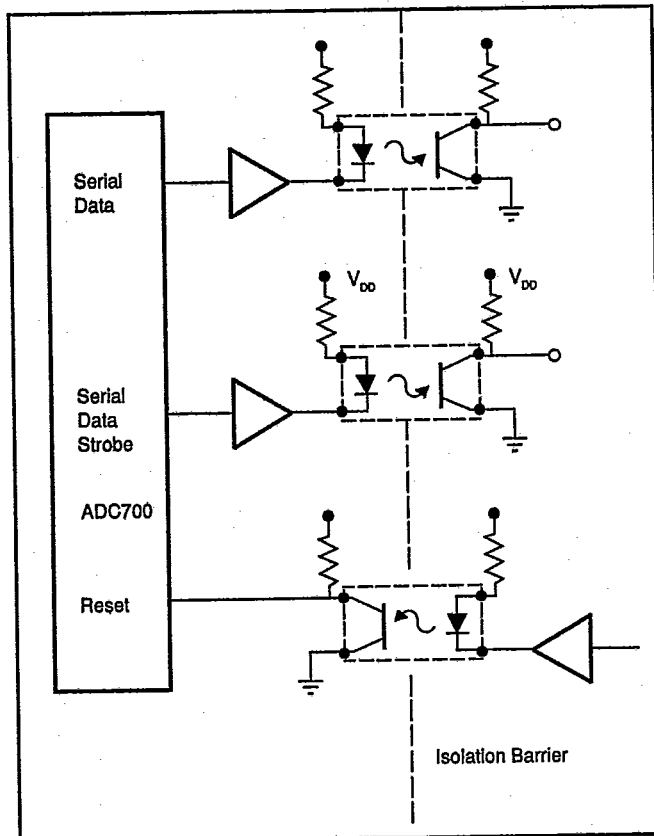
FIGURE 10. Serial Data Output Providing Convenient Isolation.
