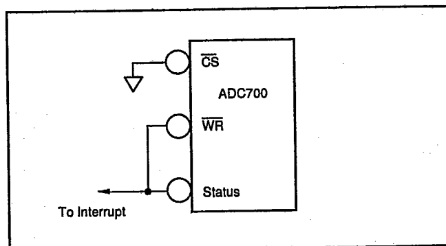
FIGURE 11. Continuous Conversion Circuit Connection.
