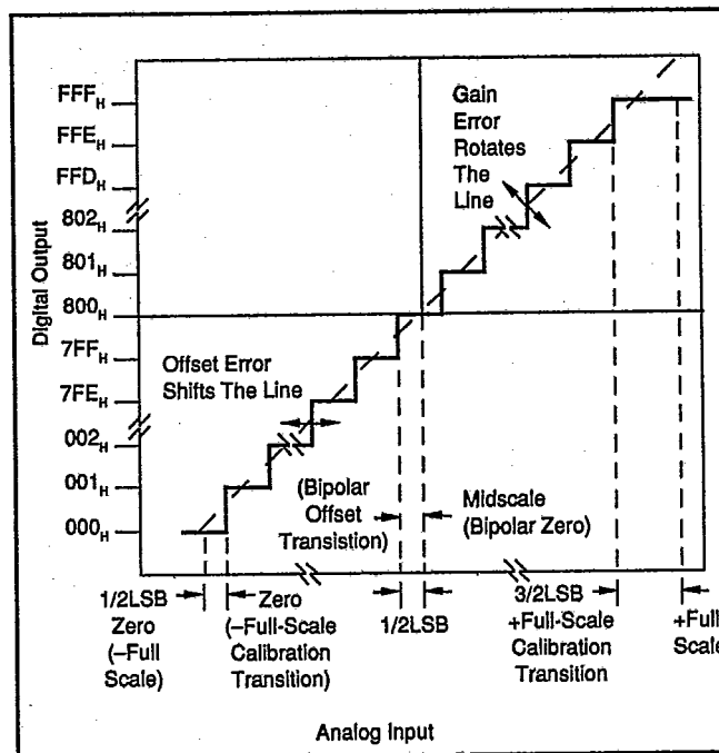
FIGURE 3. Transfer Characteristic Terminology.
