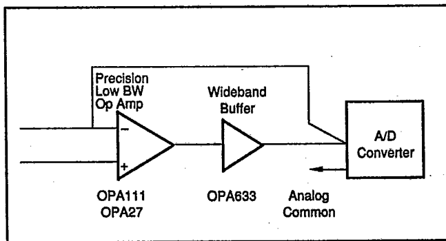
FIGURE 5. Wideband Buffer Reduces Output Impedance at High Frequencies.
