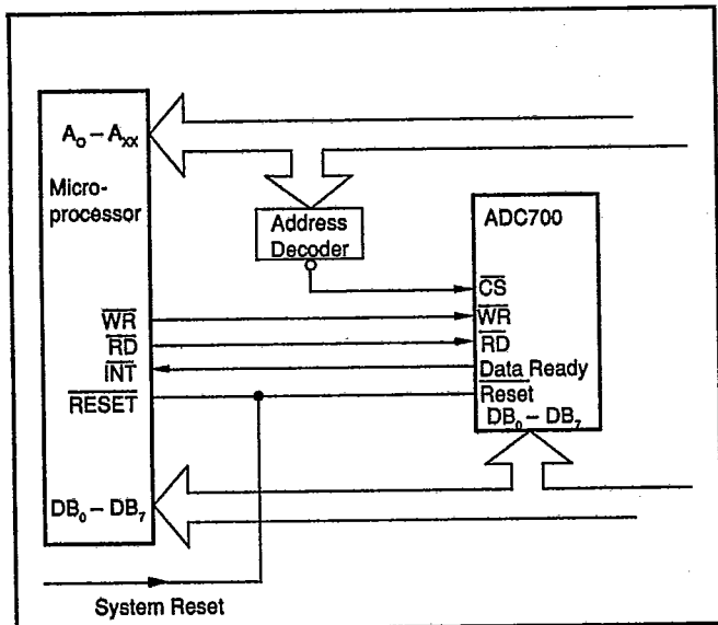
FIGURE 9. Parallel Data Bus Interface.
