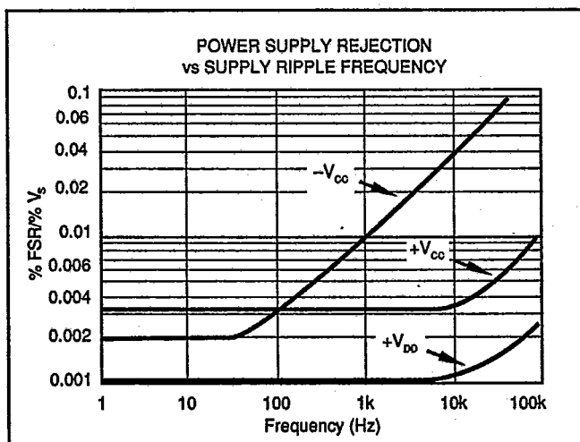
FIGURE 4. Power Supply Rejection Ripple vs Frequency.
