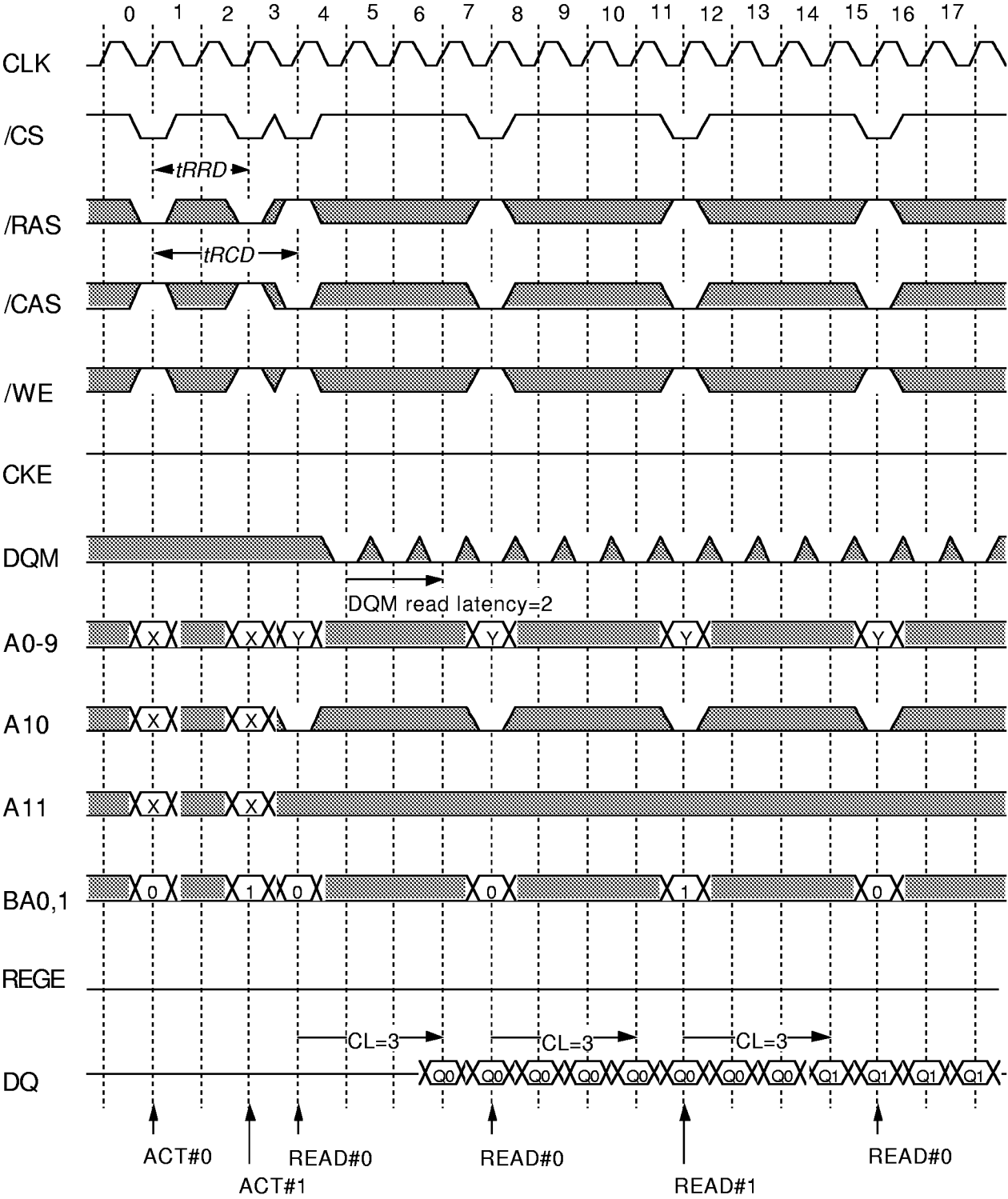
Page Mode Burst Read (multi bank) BL=4, Buffer mode(REGE="L")
