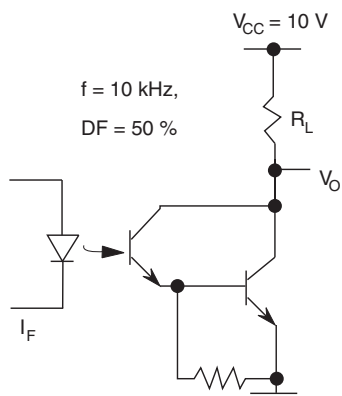
Fig. 11 - Switching Schematic
