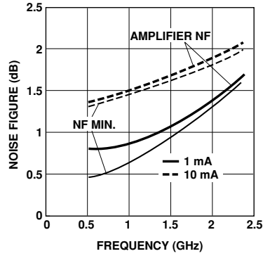
Figure 2. AT-31011 and AT-31033 Minimum Noise Figure and Amplifier \text{NF}^{(1)} vs. Frequency and Current at V_{\text{CE}} = 2.7 \text{ V} .
