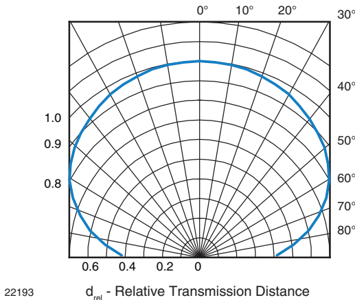
Fig. 11 - Horizontal Directivity
