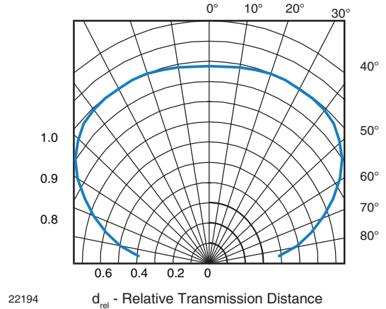
Fig. 12 - Vertical Directivity
