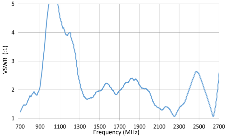
VSWR (700 - 2700 MHz)
