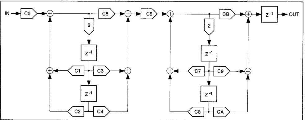
Figure G1 : Biquadratic IIR Filter
