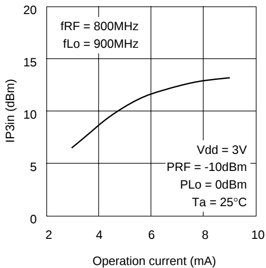
IP3in vs. Operation current
