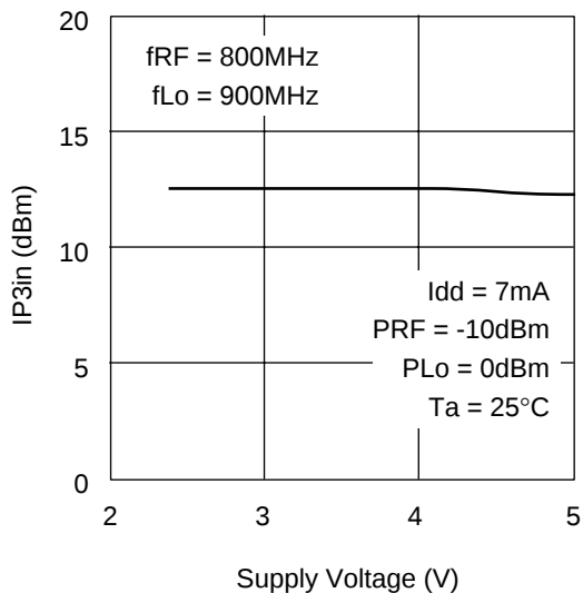
IP3in vs. Supply Voltage
