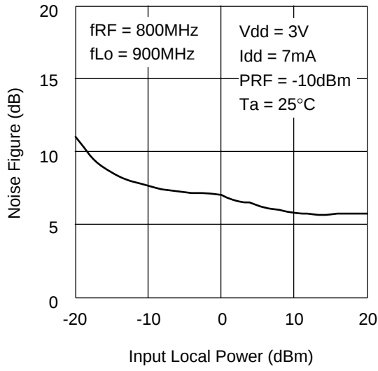
NF vs. Input Power
