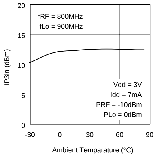
IP3in vs. Temperature
