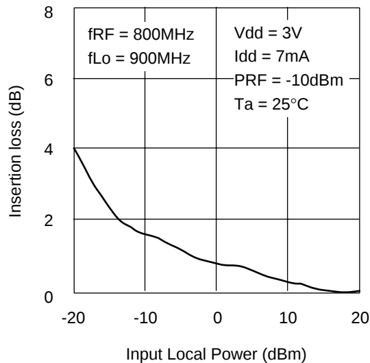
Insertion loss vs. Input Power
