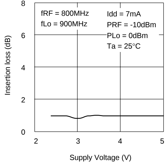
Insertion loss vs. Supply Voltage
