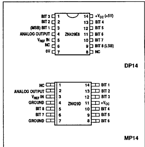
Fig.1 Pin connections (not to scale) - top view
