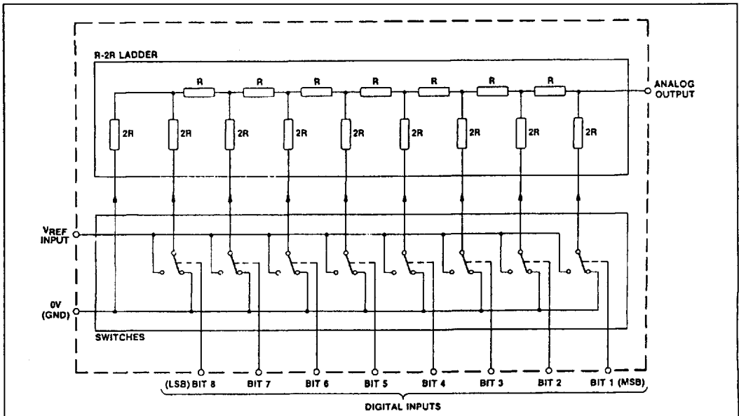
Fig.2 System diagram (see pin connection diagrams above for pin outs)
