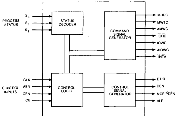
Figure 1 : CA82C88 BLOCK DIAGRAM
