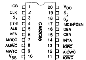
Figure 2 : PLCC and DIP PIN CONFIGURATIONS
