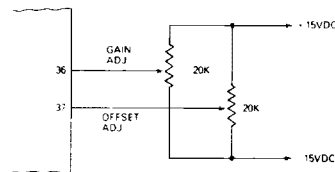
Figure 1. External Adjustment
