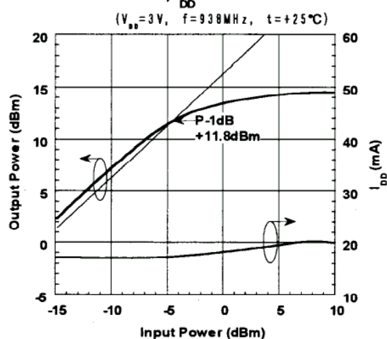
OUTPUT POWER, I DD vs. INPUT POWER
