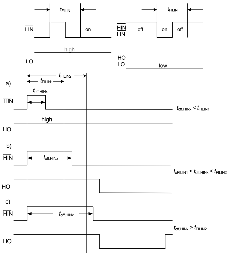
Figure E: Short Pulse suppression
