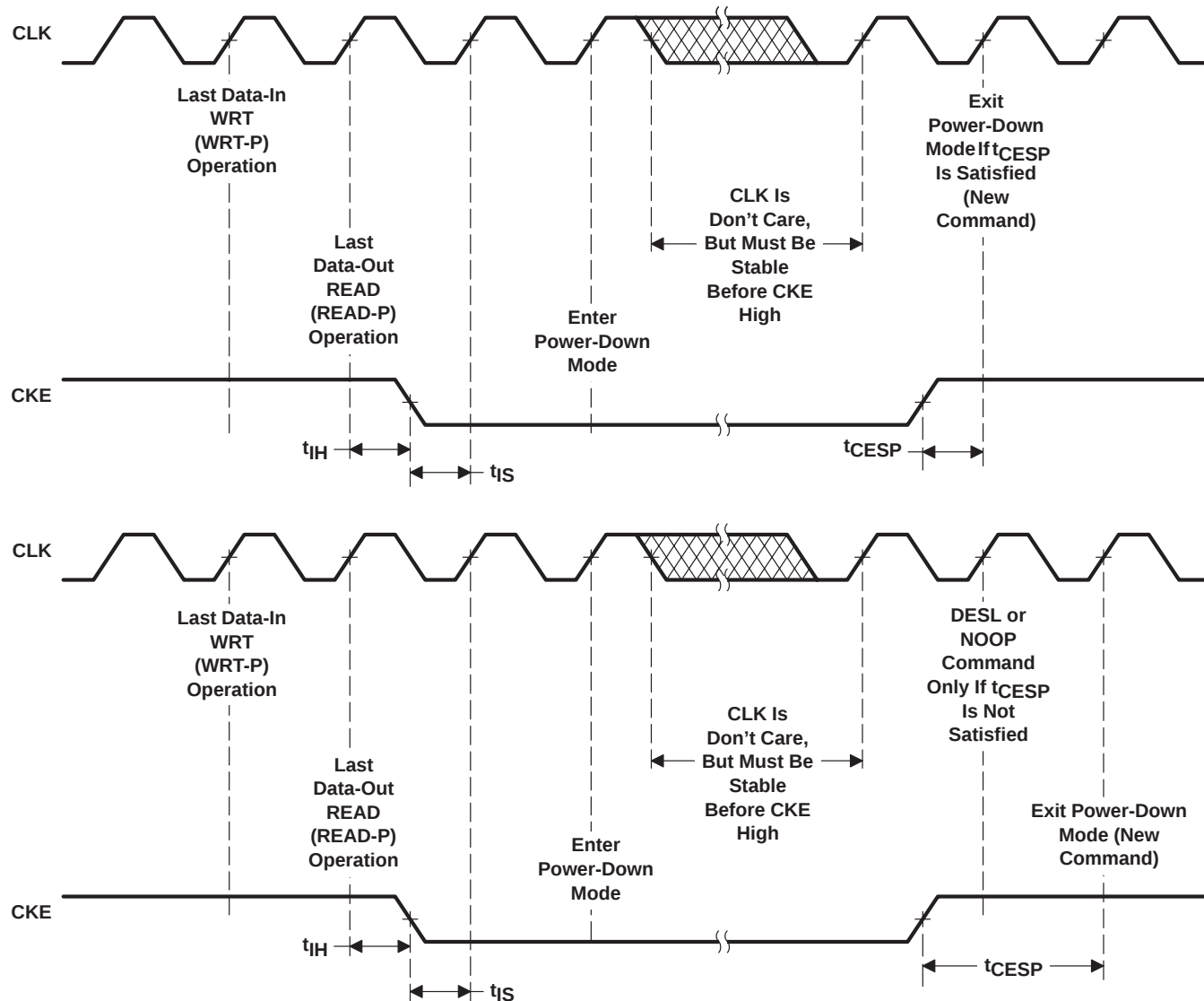
Figure 18. Power-Down Operation
