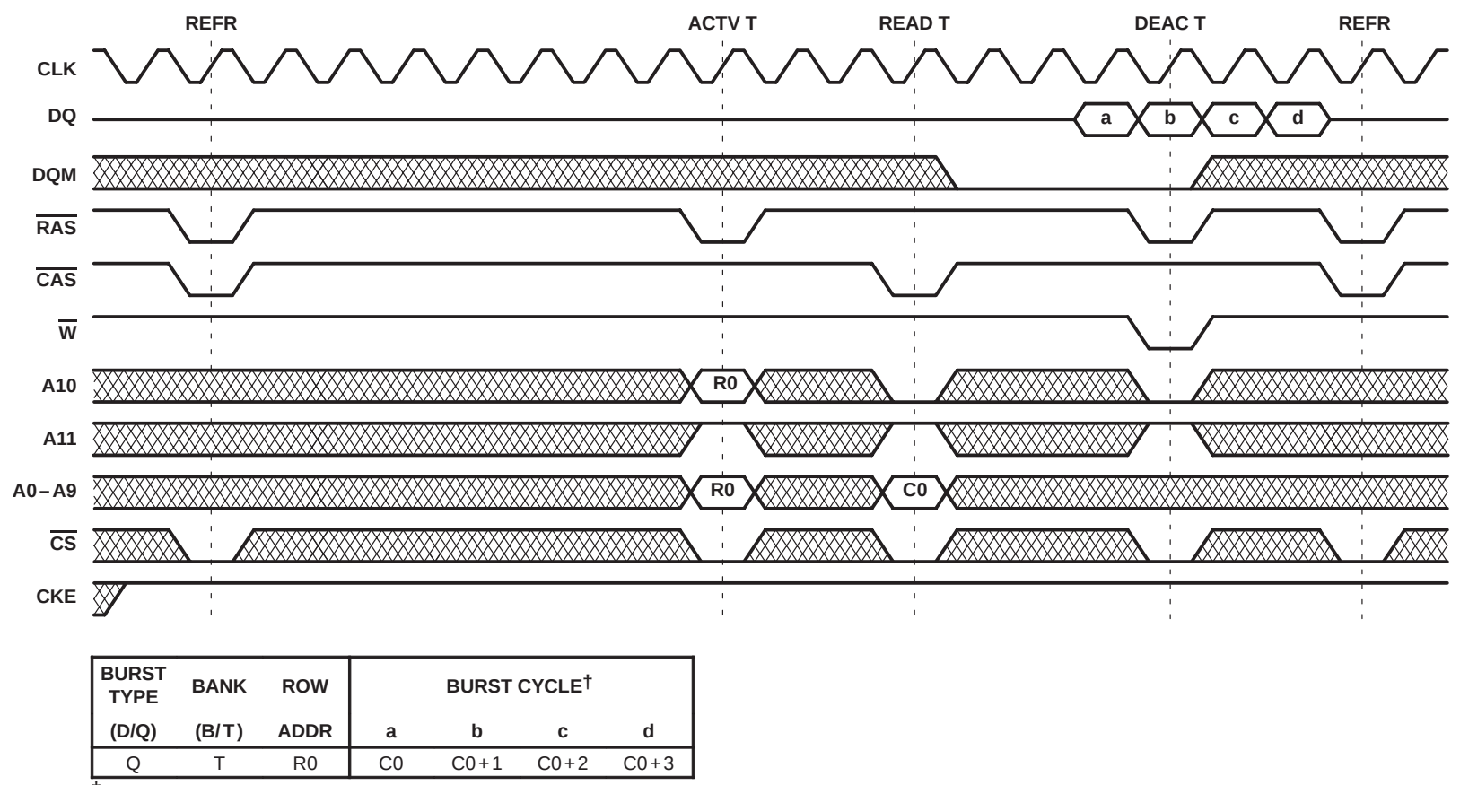
Figure 29. Refresh Cycles (CAS latency = 3, burst length = 4)
