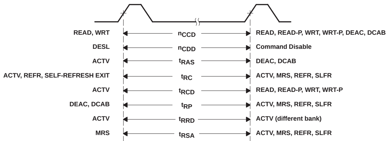
Figure 11. Command-to-Command Parameters
