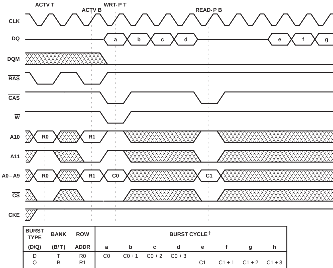
Figure 27. Write-Burst Bank T, Read-Burst Bank B With Automatic Deactivate (CAS latency = 3, burst length = 4)
