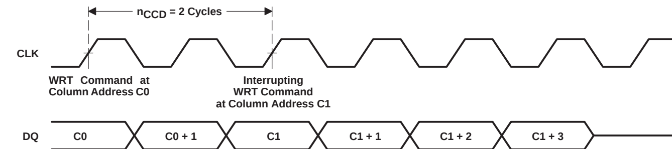
Figure 6. Write Burst Interrupted by Write Command
