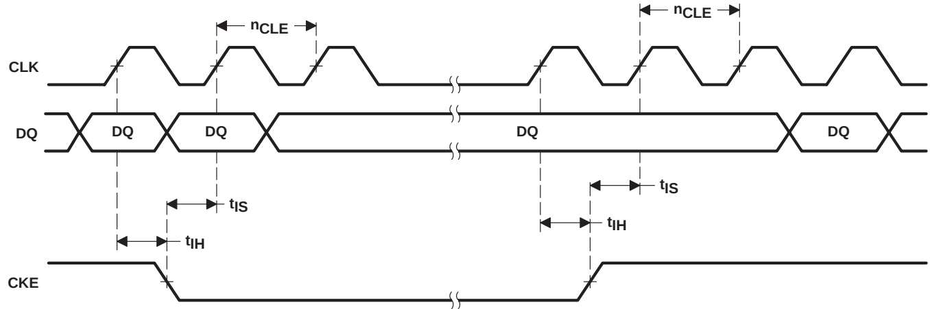
Figure 17. CLK-Suspend Operation
