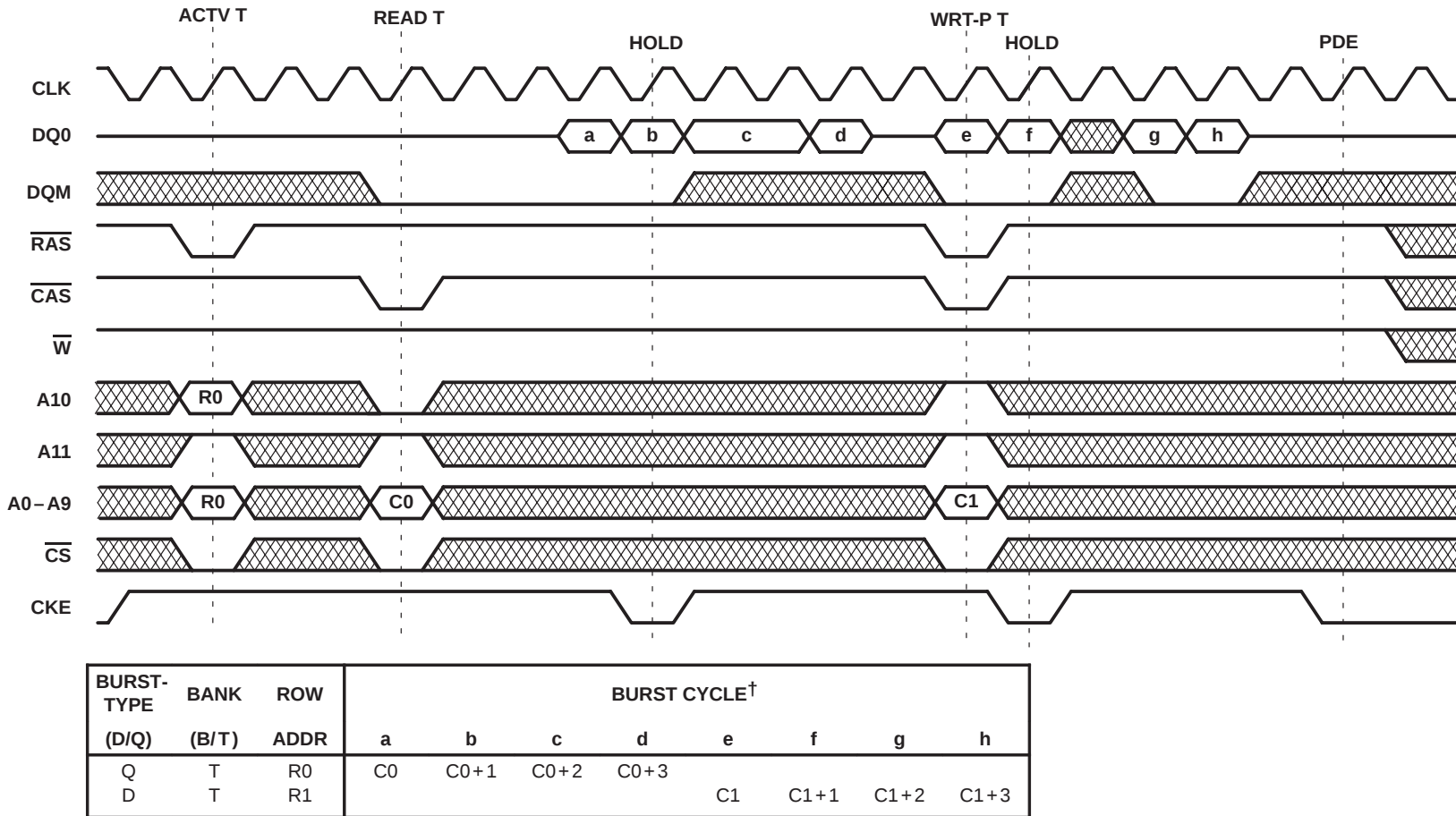
Figure 31. CLK Suspend (HOLD) During Read Burst and Write Burst (CAS latency = 3, burst length = 4)
