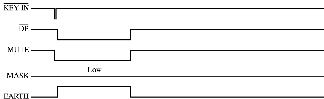
Figure 11. Symbolic timing diagram: Earth function
