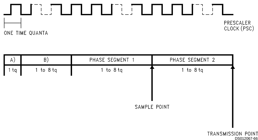
FIGURE 31. Bit Timing
