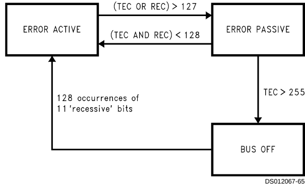
FIGURE 30. CAN Bus States
