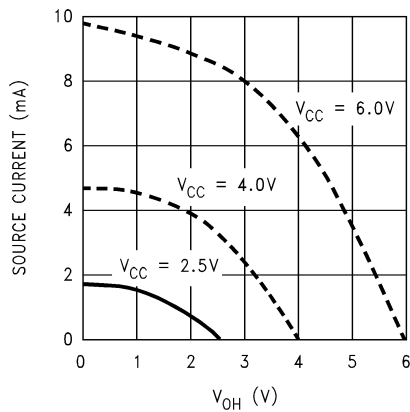
Ports G/L Source Current
