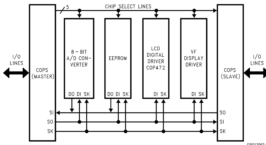
FIGURE 39. MICROWIRE/PLUS Application
