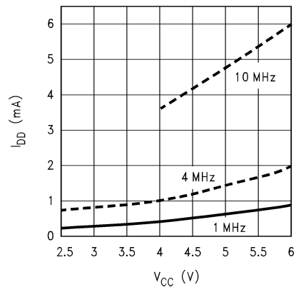
Dynamic I_{DD} vs V_{CC}
