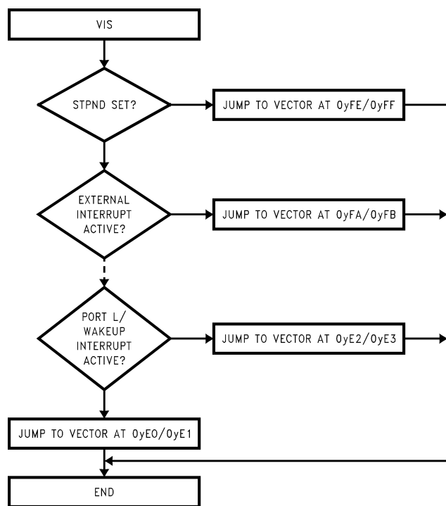
FIGURE 37. VIS Flowchart
