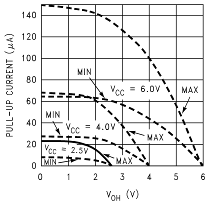
Ports G/L Weak Pull-Up Source Current
