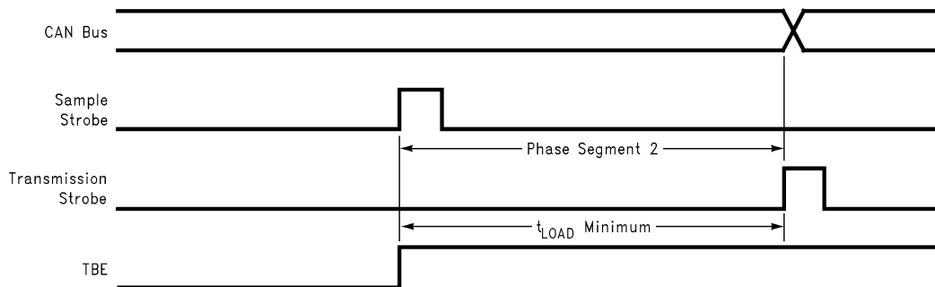
FIGURE 19. TBE Timing
