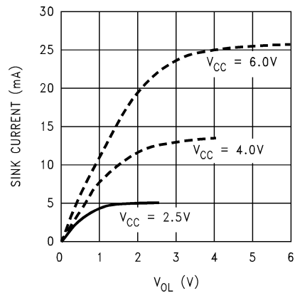
Port G/L Sink Current
