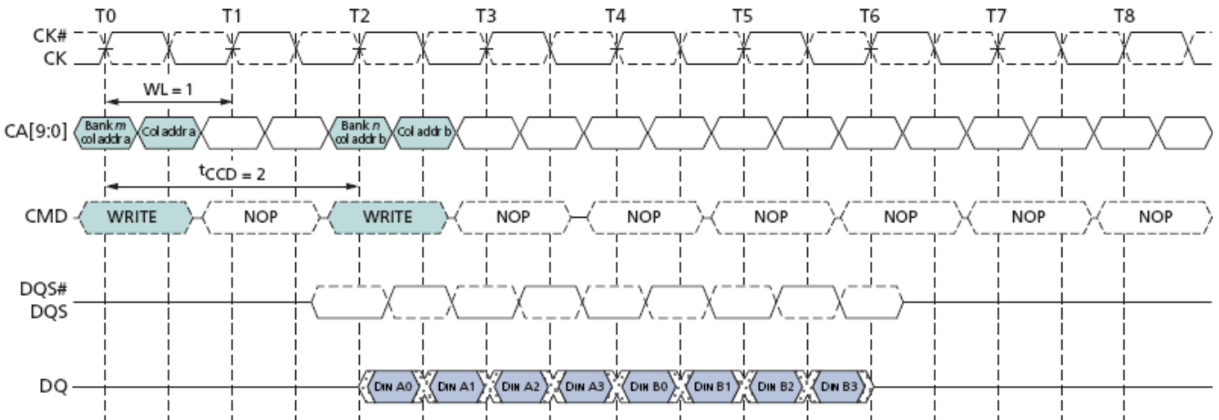
Seamless Burst write: WL=1, BL=4, Tccd=2
