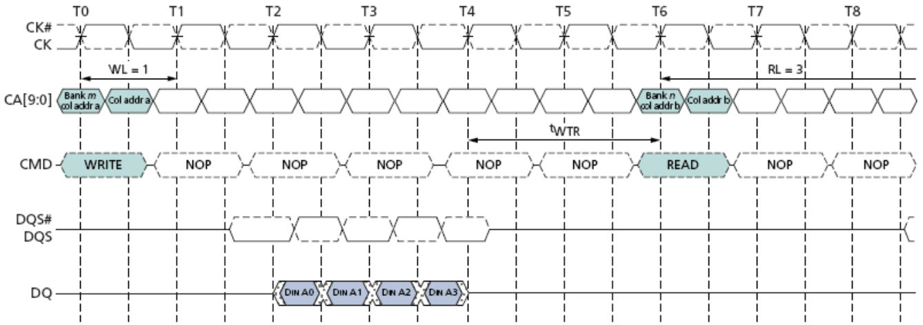
Burst write followed by burst read: RL=3, WL=1, BL=4
