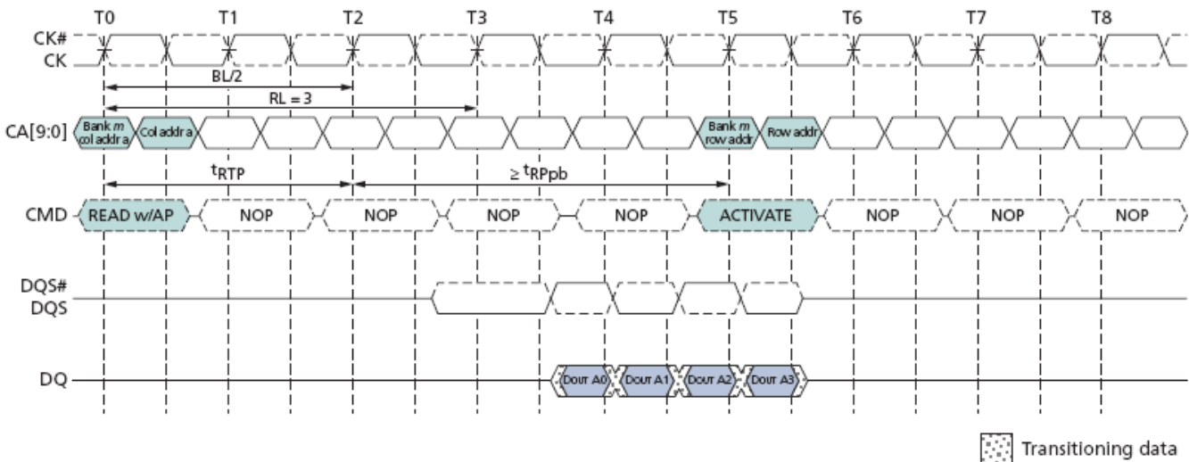
Burst Read with Auto-Precharge: RL=3, BL=4, RU(\text{RTP}(\text{min})/\text{CK})=2
