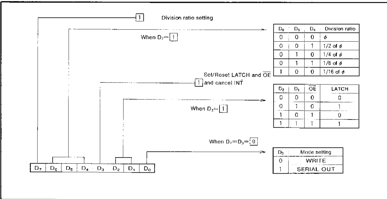
Fig. 2 Instruction set
