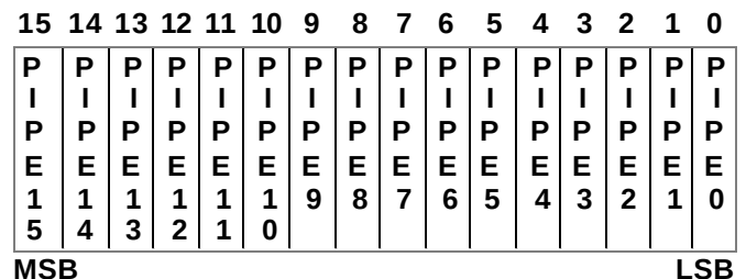
Figure 21. The PIPE Register (PIPE)
