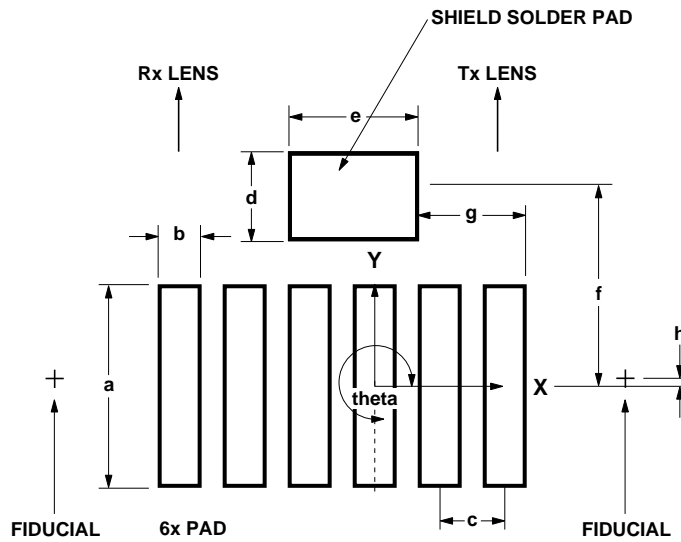
Figure 2. Top view of land pattern.
