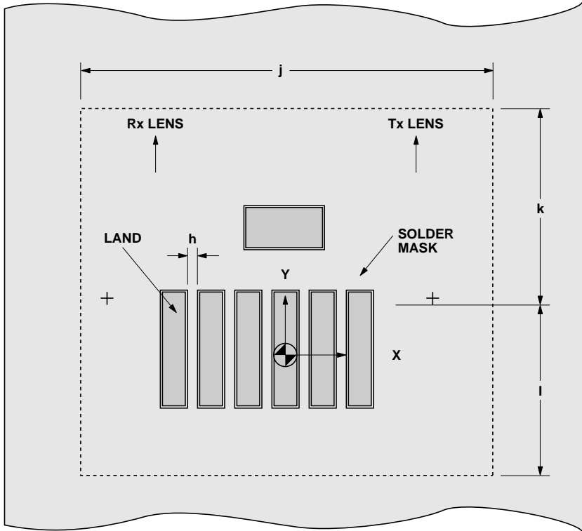
Figure 3. HSDL-3001#007/#017 PCBA – adjacent land keep-out and solder mask.
