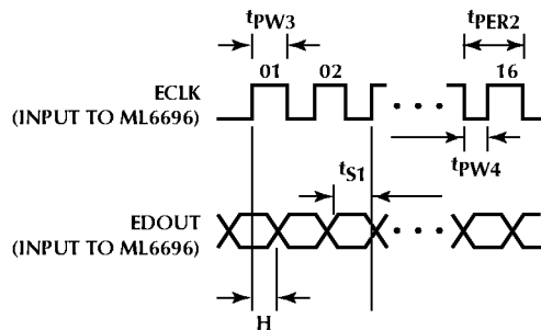
Figure 6. MII Management Interface Read Timing
