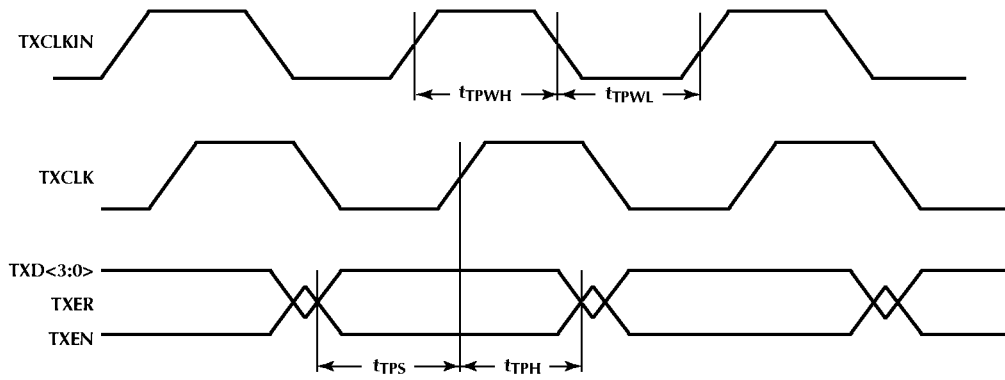
Figure 1. MII Transmit Timing
