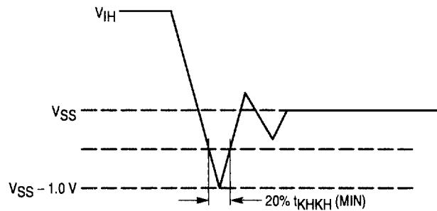
Figure 1. Undershoot Voltage
