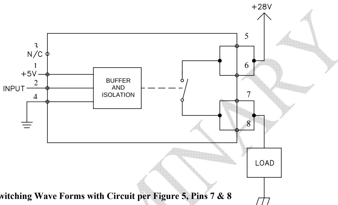
Figure 5: Typical Application
