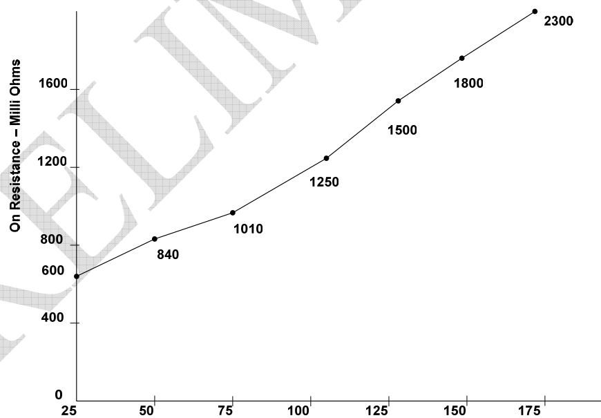
Figure 4: Typical On Resistance as a Function of Junction Temperature
