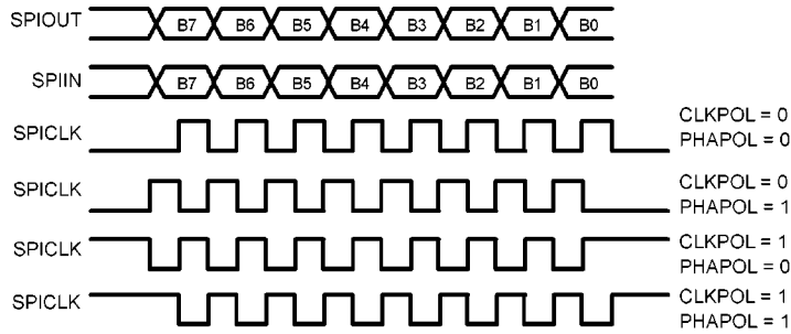
Figure 14-3 CLKPOL/PHAPOL Timing
