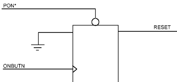
Figure 12-1 Reset Flip-Flop
