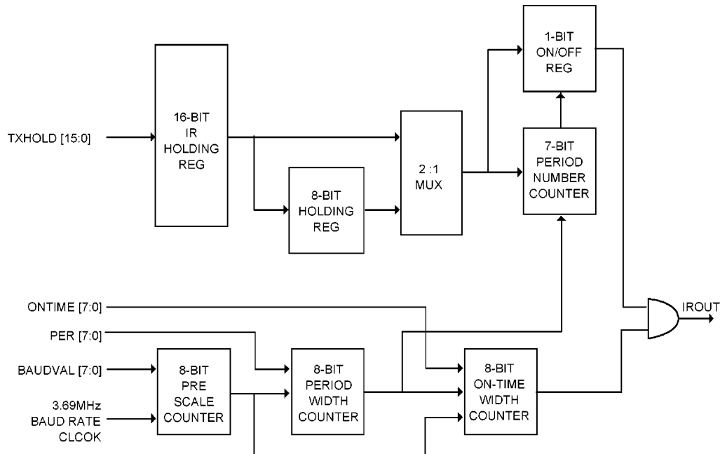
Figure 10-2 Consumer IR Block Diagram
