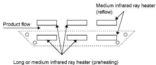
Figure 1.1.2 Heating Top and Bottom with Long or Medium Infrared Rays
