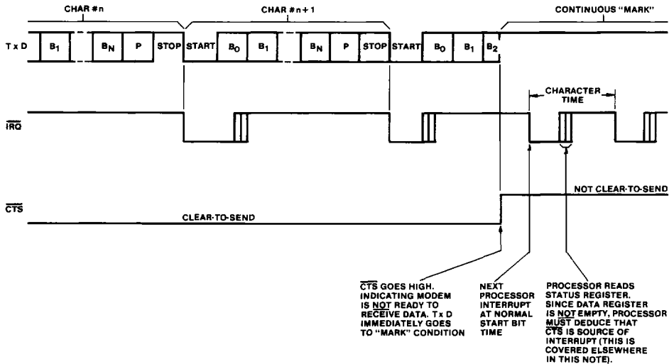
Fig. 11 - Effect of \overline{\text{CTS}} on transmitter.
