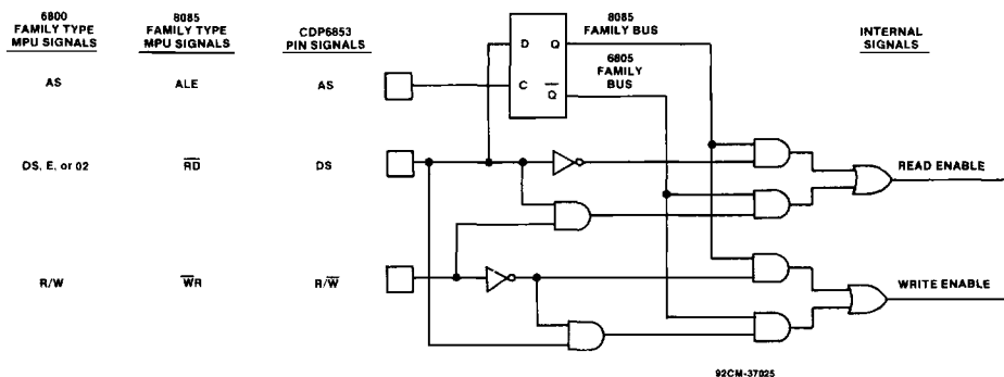
Fig. 2 - Functional diagram of MOTEL circuit.
