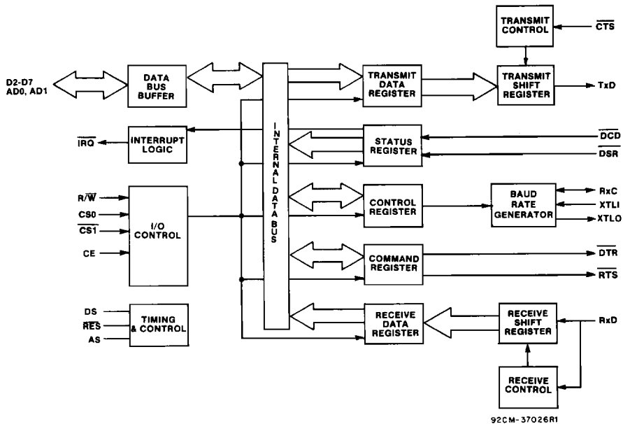
Fig. 3 - Internal organization.
