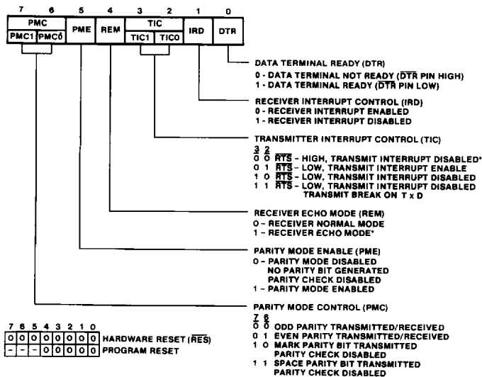
Fig. 6 - CDP6853 command register.
