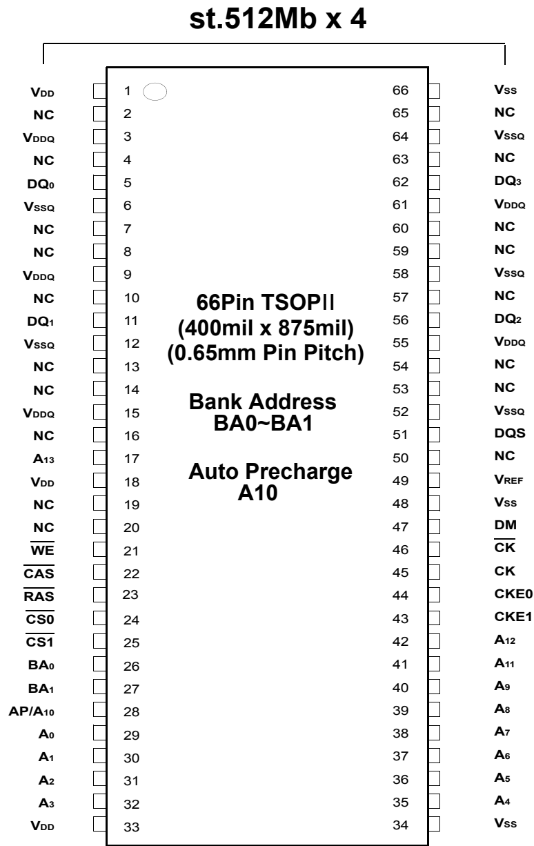
stacked 2Gb TSOP-II Package Pinout
