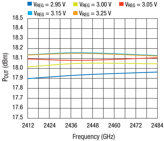
V_{REG} vs. P_{OUT} OFDM Modulation, 54 Mbps, V_{CC} = 3.3 V, T_A = 25 °C
