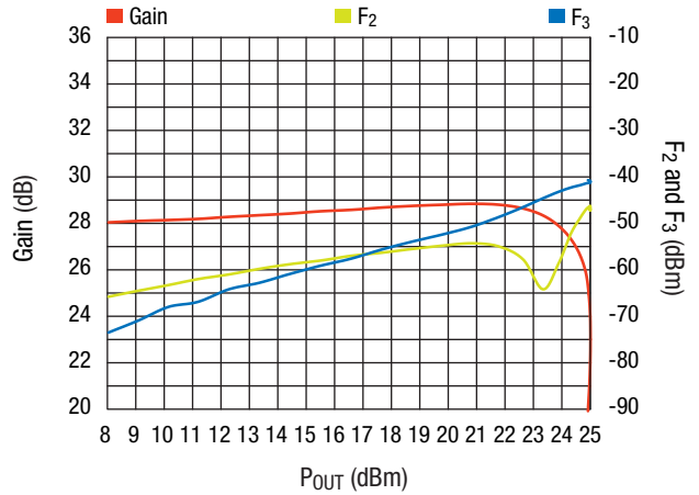
CW, 2F and 3F Harmonics vs. P_{OUT} V_{CC} = 3.3 V, V_{REG} = 3 V, F_C = 2.442 GHz, T_A = 25 °C
