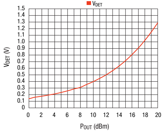
V_{DET} vs. P_{OUT} OFDM Modulation, 54 Mbps, V_{CC} = 3.3 V, V_{REG} = 3 V, F_C = 2.442 GHz, T_A = 25 °C
