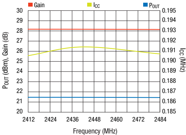
802.11b P_{OUT} , Gain, and I_{CC} vs. Frequency CCK Modulation, 11 Mbps, V_{CC} = 3.3 V, T_A = 25 °C
