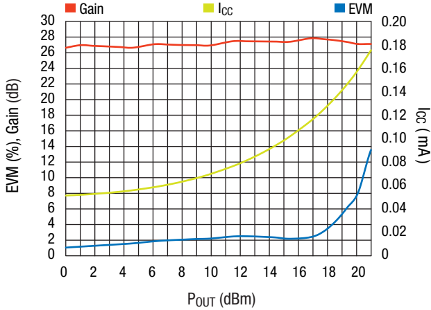
802.11g EVM and I_{CC} vs. P_{OUT} OFDM Modulation, 54 Mbps, V_{CC} = 3.3 V, V_{REG} = 3 V, F_C = 2.442 GHz, T_A = 25 °C
