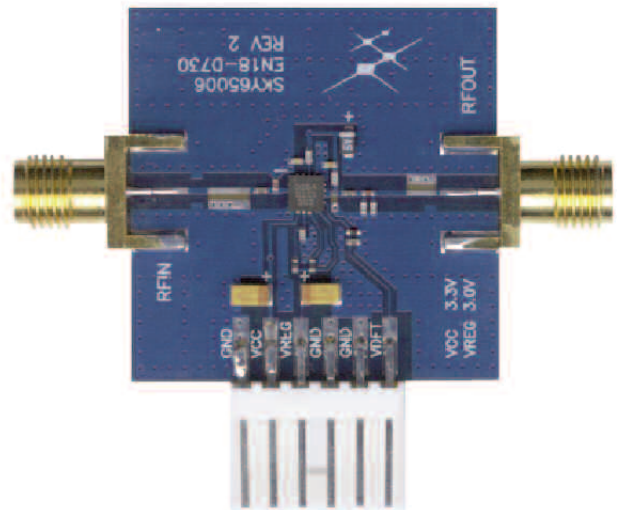
Board Photograph
