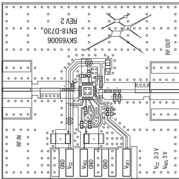
Board Layout
