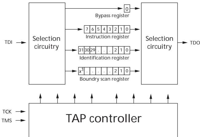
Figure 42: TAP Controller Block Diagram
