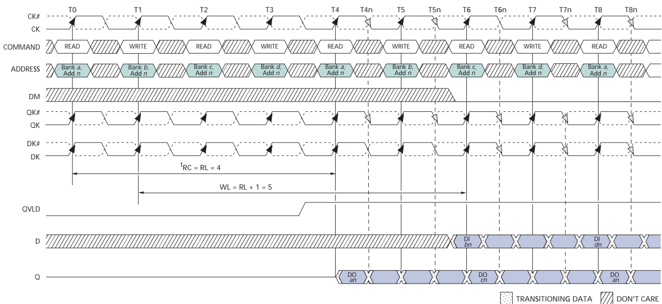
Figure 27: READ/WRITE Interleave
