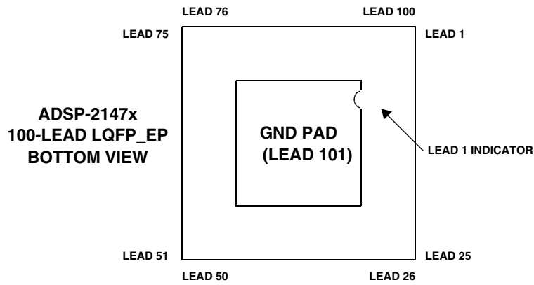
Figure 54. 100-Lead LQFP_EP Lead Configuration (Bottom View)
