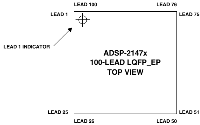
Figure 53. 100-Lead LQFP_EP Lead Configuration (Top View)
