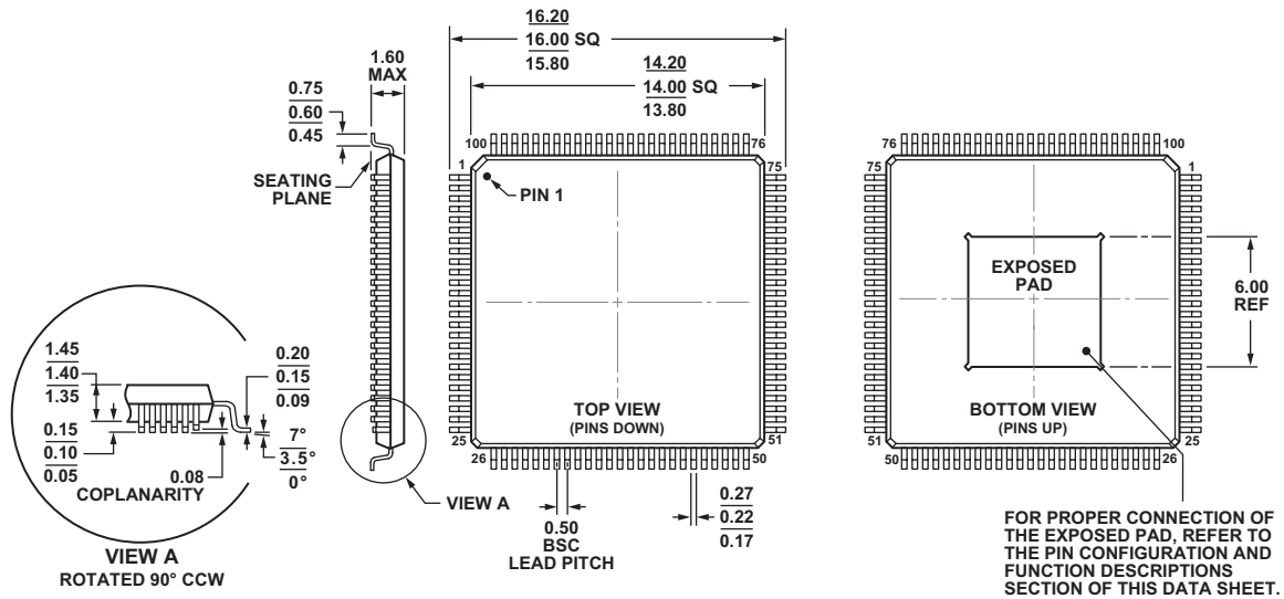
Figure 55. 100-Lead Low Profile Quad Flat Package, Exposed Pad [LQFP_EP] (SW-100-2)
