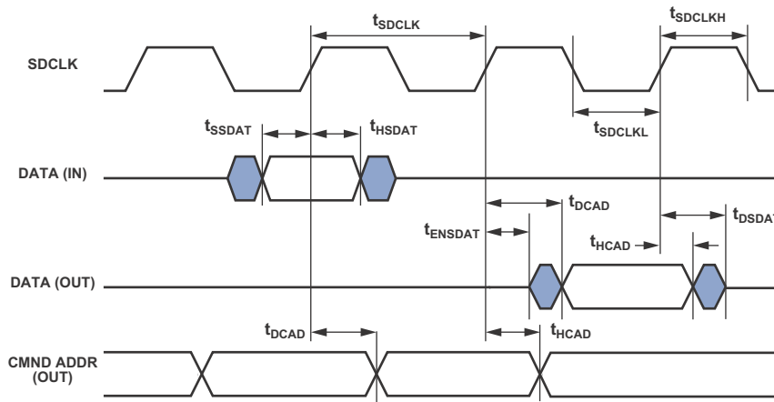
Figure 19. SDRAM Interface Timing
