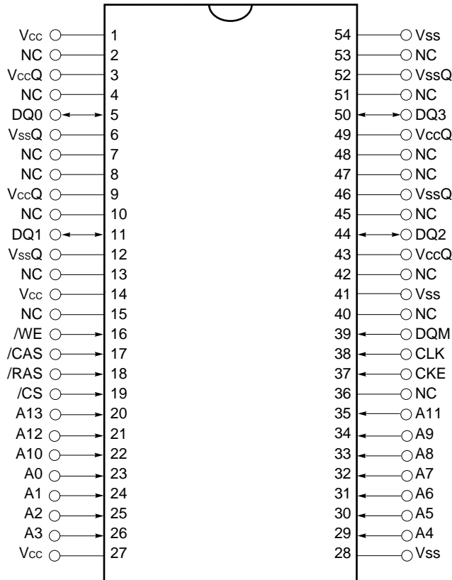
[ μPD4564441-A75 ] 54-pin Plastic TSOP (II) (400 mil) 4M words × 4 bits × 4 banks
