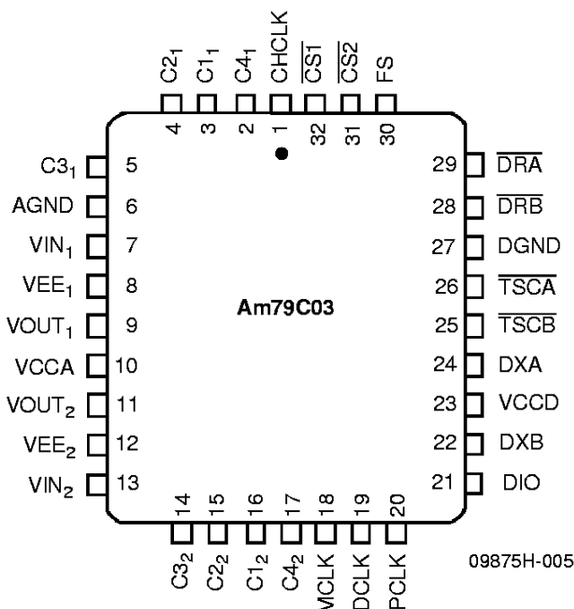
32-Pin PLCC
