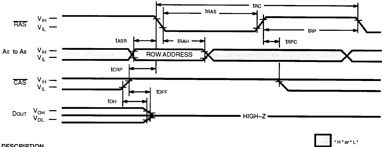
Fig. 10 – \overline{\text{RAS}} -ONLY REFRESH CYCLE
