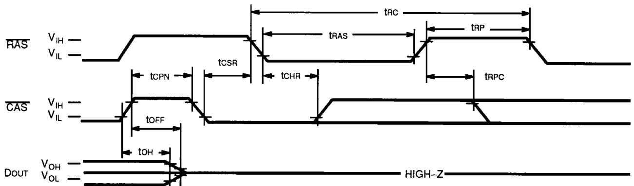
Fig. 11 – \overline{\text{CAS}} -BEFORE- \overline{\text{RAS}} REFRESH CYCLE
