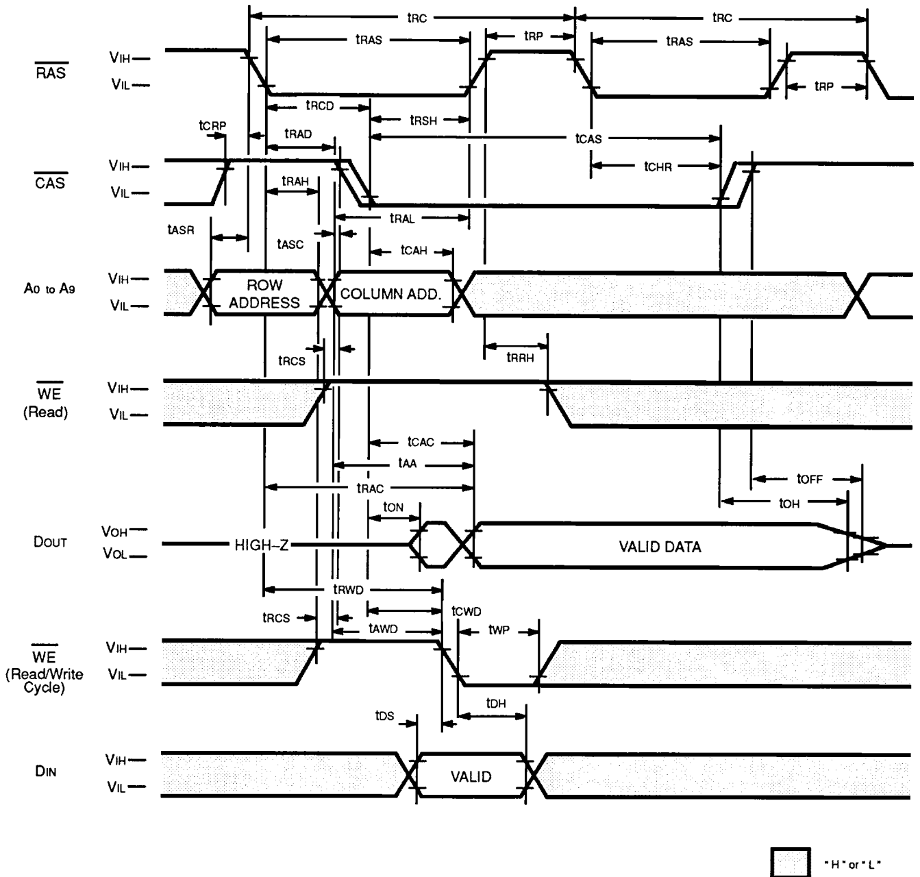
Fig. 12 – HIDDEN REFRESH CYCLE
