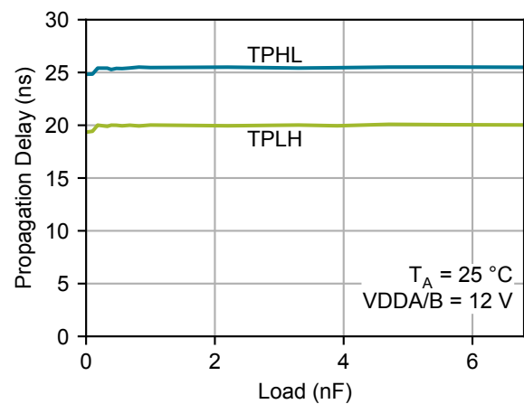
Figure 4.6. Propagation Delay vs. Load
