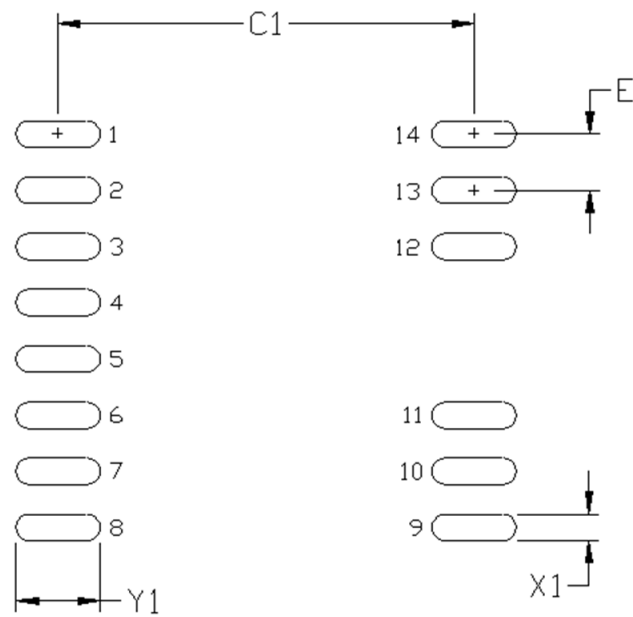
Figure 8.1. 14-Pin WB SOIC Land Pattern
