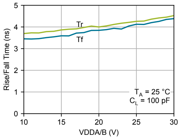
Figure 4.3. Rise/Fall Time vs. Supply Voltage
