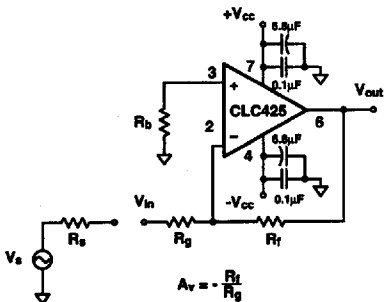
Figure 2: Inverting Amplifier Configuration
