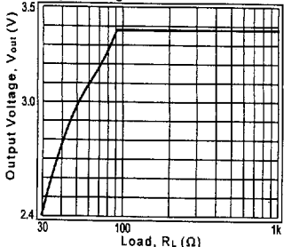
Output Voltage vs Load
