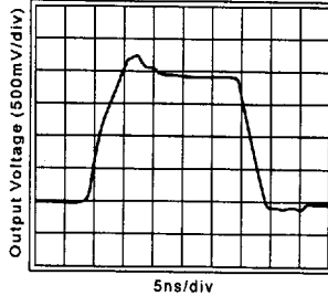
Long Term Settling Time
