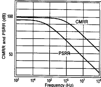
CMRR and PSRR
