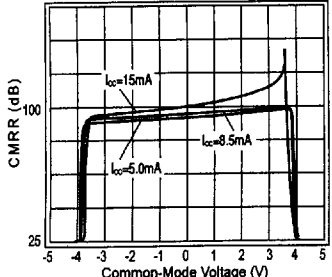
CMRR vs Common-Mode Input Voltage
