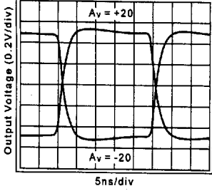
Short Term Settling Time
