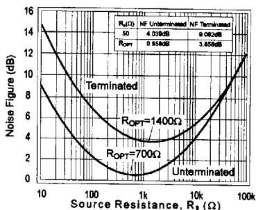
Figure 6: Noise Figure vs Source Resistance
