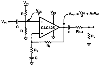
Figure 10: Single Supply Operation
