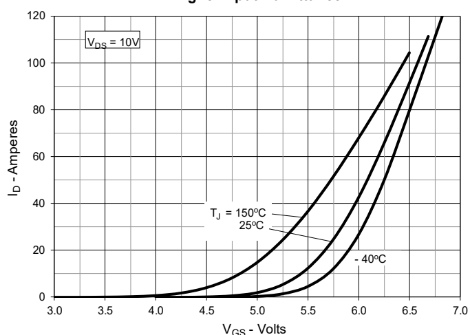
Fig. 8. Input Admittance
