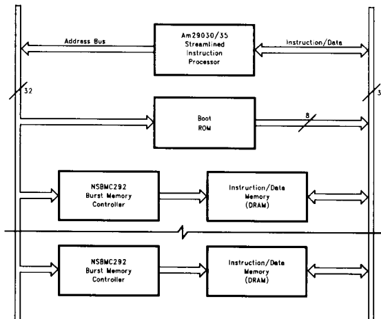
Typical System Configuration
