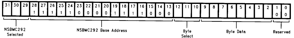
FIGURE 2. Address Bus Fields Used to Access Configuration Data
