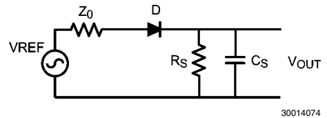
FIGURE 2. Diode Detector
