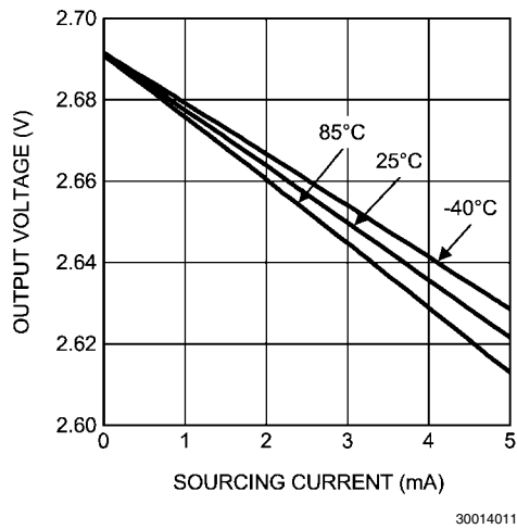
Output Voltage vs. Sourcing Current
