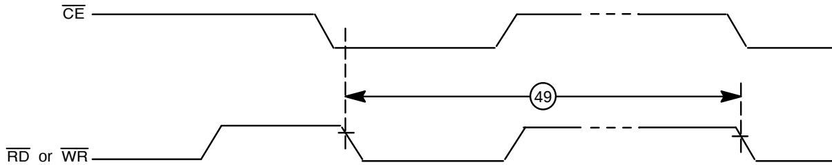
Figure 22. Reset Timing
