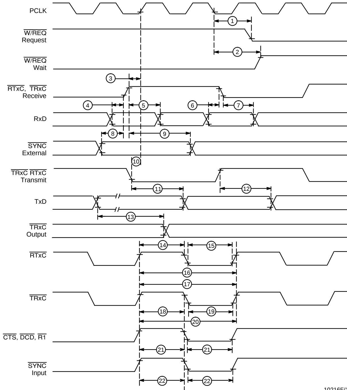
Figure 19. General Timing
