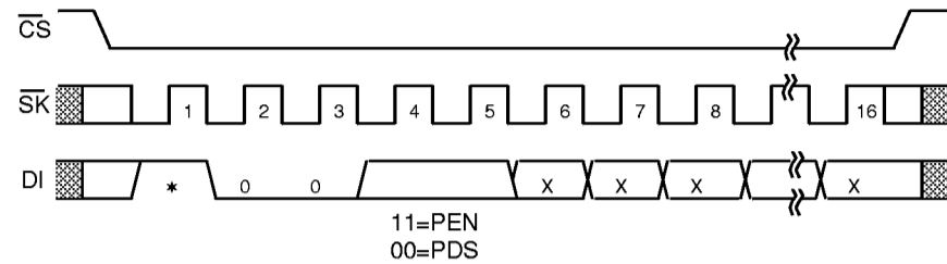
Figure 7 PEN/PDS Timing
