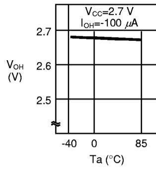
1.18 High level output voltage V_{OH} – Ambient temperature T_a
