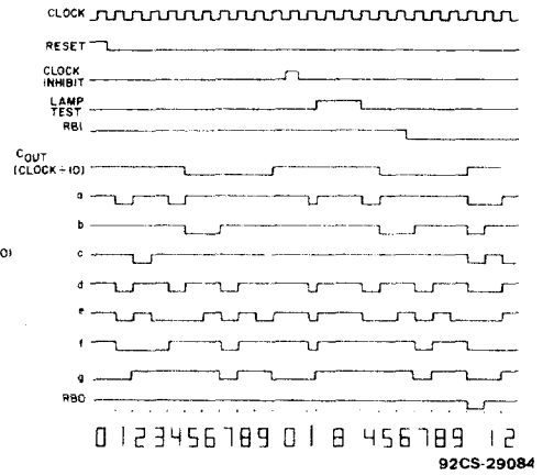
Fig. 4 - CD4033B timing diagram.
