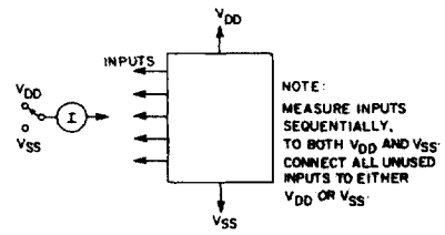
Fig. 17 - Input current.
