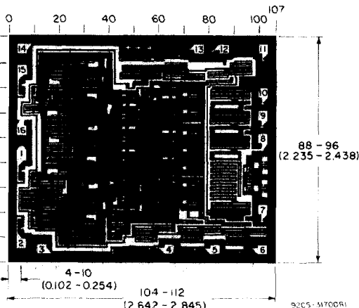
Dimensions and pad layout for CD4026B.
