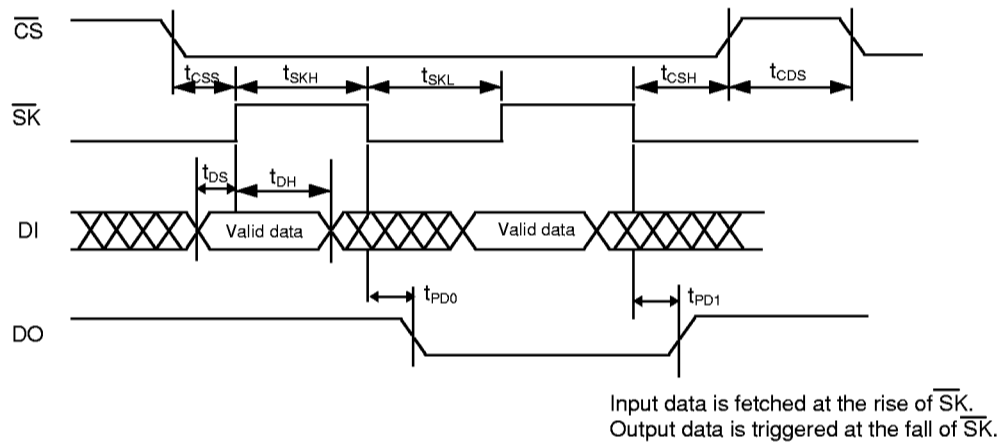
Figure 3 Timing chart
